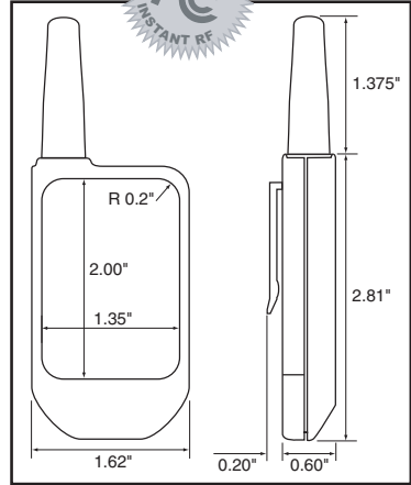
PHYSICAL DIMENSIONS
