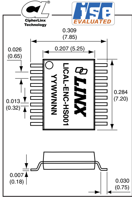
PHYSICAL DIMENSIONS
