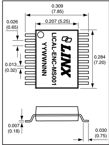
PHYSICAL DIMENSIONS
