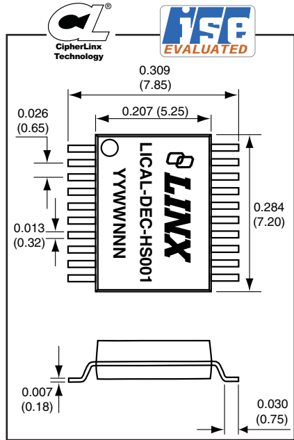
PHYSICAL DIMENSIONS
