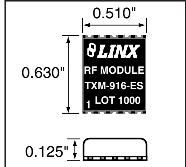
PHYSICAL DIMENSIONS
