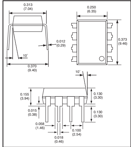
PHYSICAL DIMENSIONS
