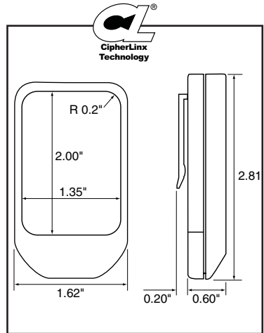
PHYSICAL DIMENSIONS
