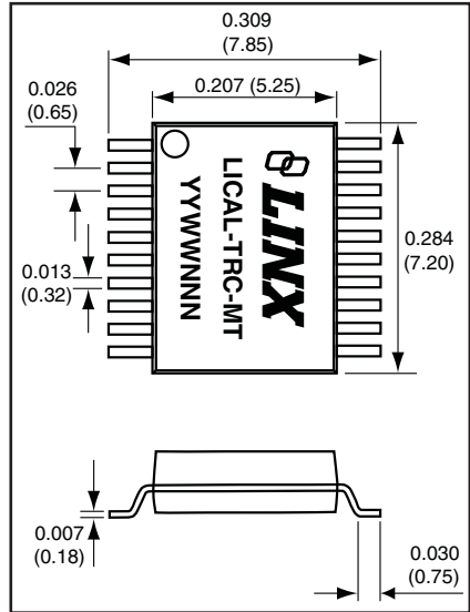
PHYSICAL DIMENSIONS
