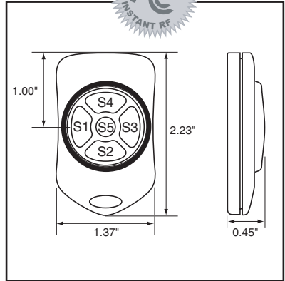
PHYSICAL DIMENSIONS
