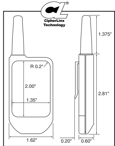
Figure 1: Package Dimensions
