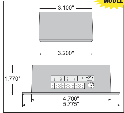
PHYSICAL DIMENSIONS
