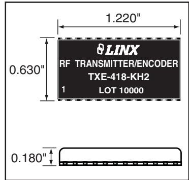
PHYSICAL DIMENSIONS
