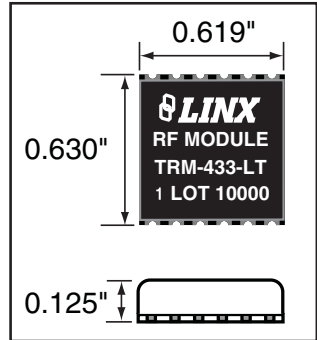
PHYSICAL DIMENSIONS
