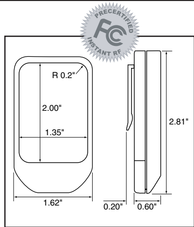
PHYSICAL DIMENSIONS
