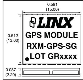
PHYSICAL DIMENSIONS
