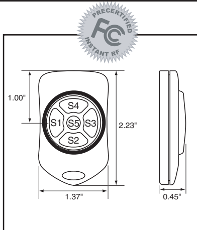
PHYSICAL DIMENSIONS
