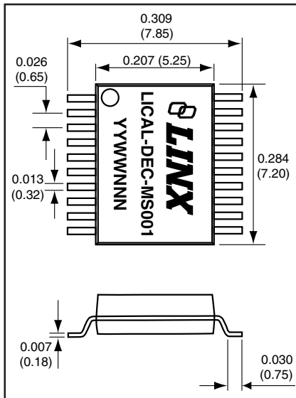
PHYSICAL DIMENSIONS
