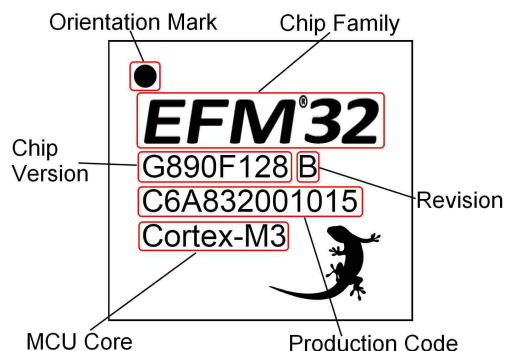
Figure 6.1. QFN64 Chip Marking
