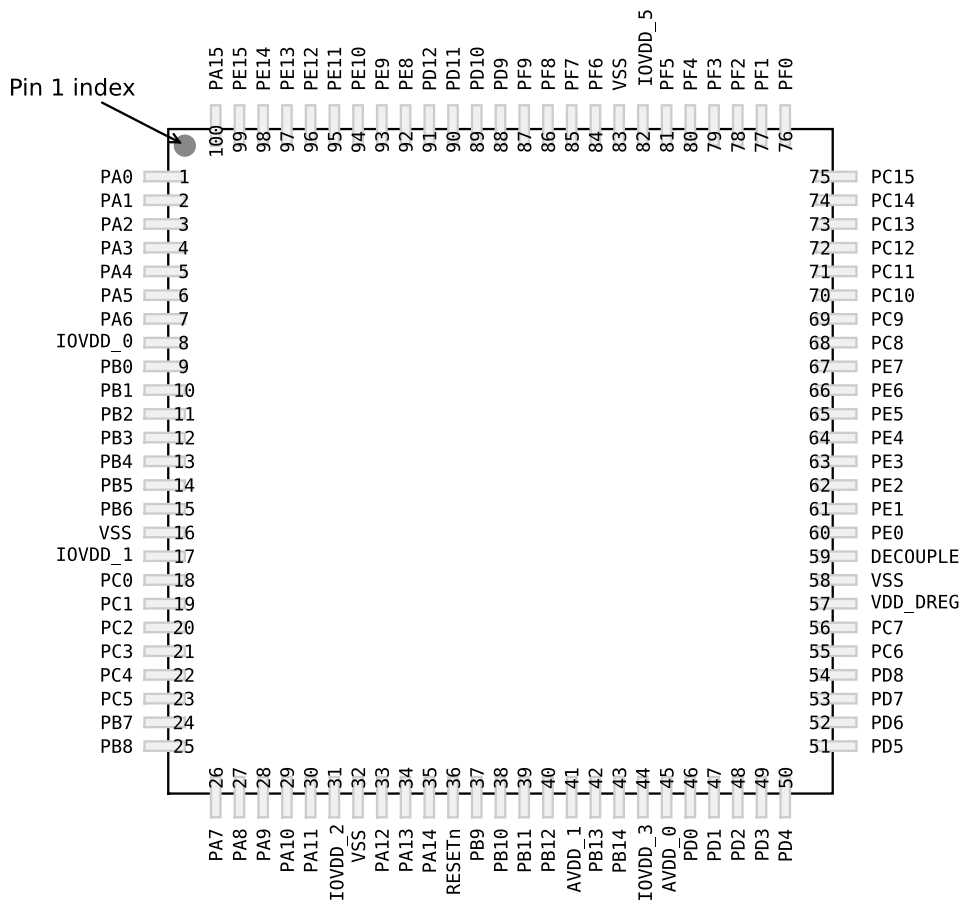
Figure 4.1. EFM32G880 Pinout (top view, not to scale)
