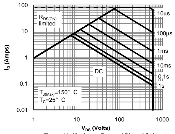
Figure 10: Maximum Forward Biased Safe Operating Area for AOTF11C60 (Note F)
