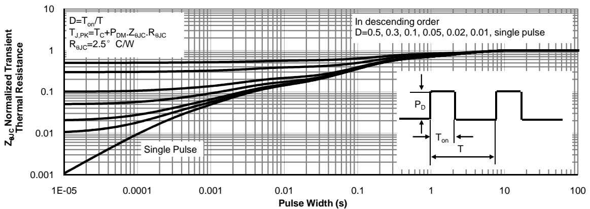
Figure 11: Normalized Maximum Transient Thermal Impedance for AOTF11C60 (Note F)
